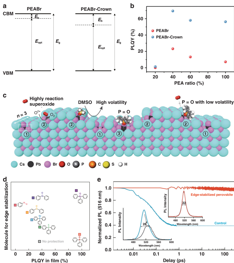
Fig. 4 Additive engineering for high-efficiency and stable quasi-2D perovskite films. a Energy schematic diagram of 40% PEABr with and without a “crown” additive. b PLQY versus PEABr ratio for the quasi-2D perovskite films with and without the “crown” additive. c Schematic illustrating imperfect edges of \text{PEA}_2\text{Cs}_2\text{Pb}_3\text{Br}_{10} perovskite films and the reaction pathway to produce superoxide under photoexcitation. d Corresponding PLQYs of quasi-2D perovskite films treated with different molecules. e PL stability for the control (blue) and edge-stabilized (red) quasi-2D perovskites before and after (in gray) measurement. Panels a and b are reprinted from ref. 78 with permission from Springer Nature. Panels c–e are reprinted from ref. 79 with permission from Springer Nature
